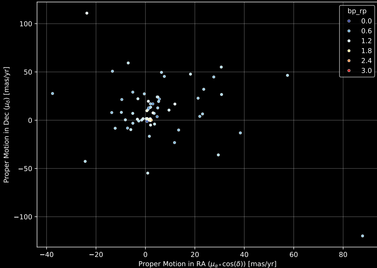
APOGEE DR17 Field: [280-33-O] Proper Motion Diagram (n= 158)
