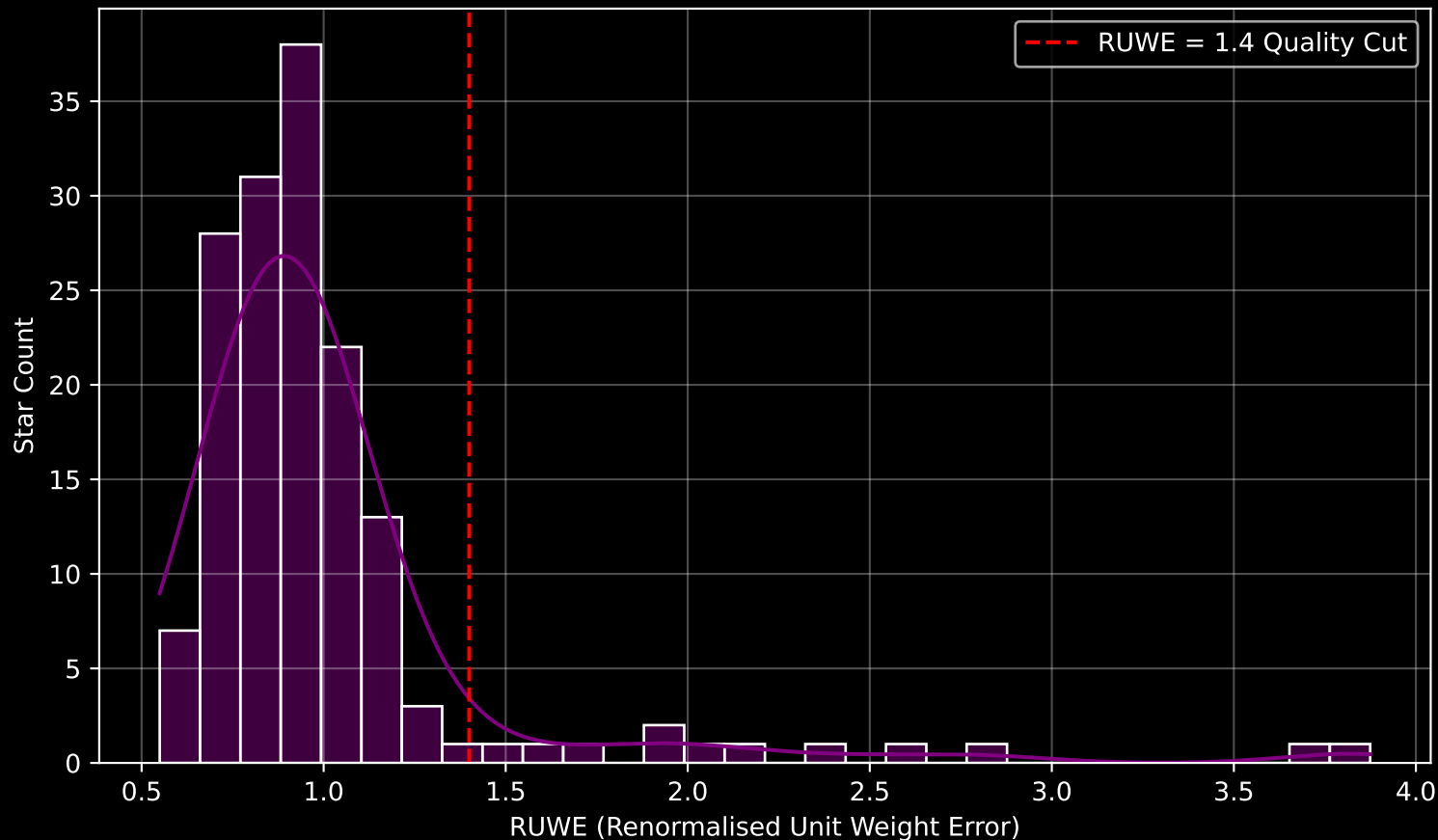
GAPOGEE DR17 Field [280-33-O] RUWE Distribution (n= 155)
