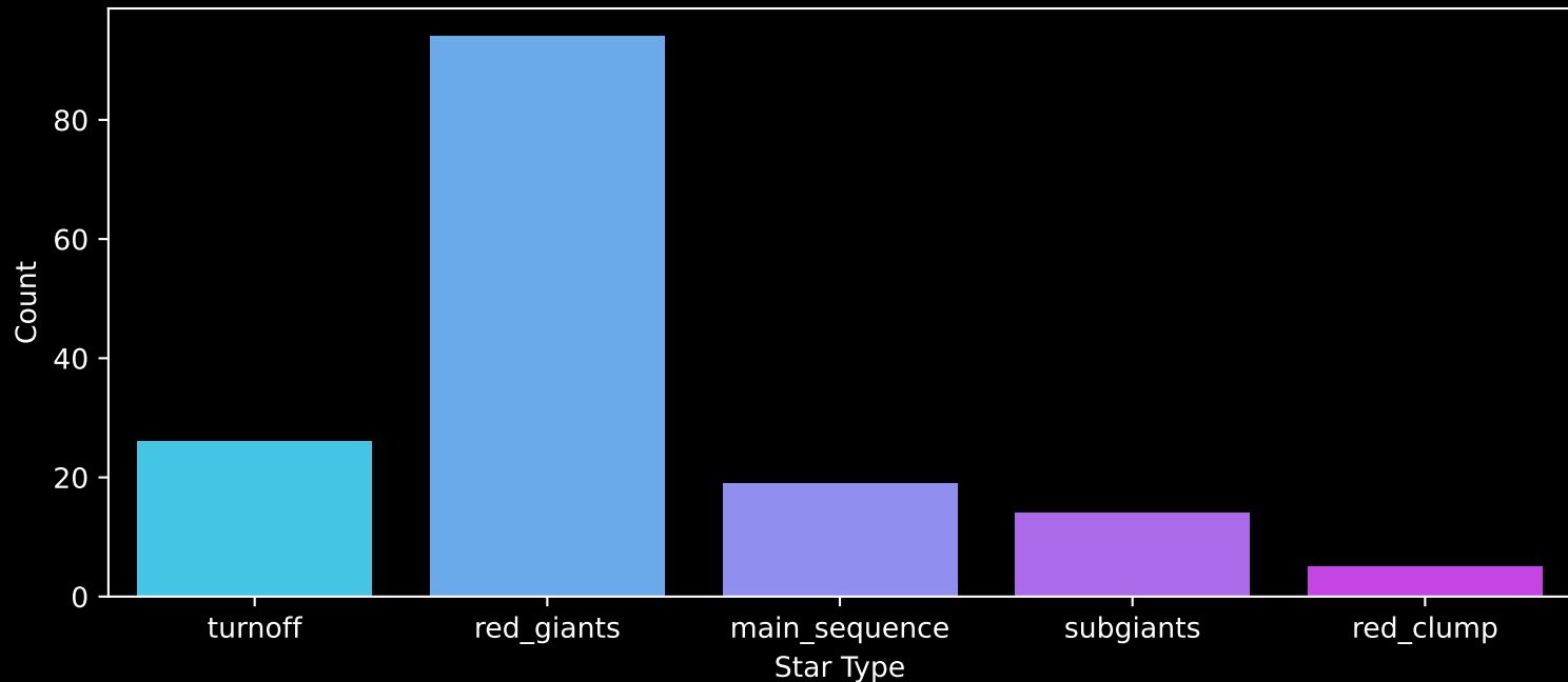
APOGEE DR17 Field: [280-33-O] Count plot of Star Type
