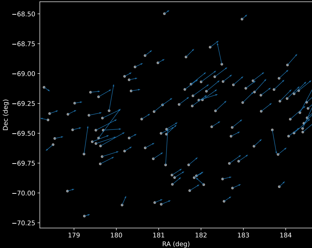
APOGEE DR17 Cluster 0 Proper Motion Vectors (n=105)
