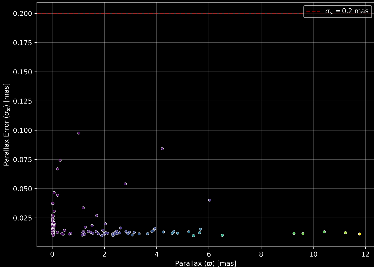
APOGEE DR17 Field: [280-33-O] Parallax Quality (n= 158)
